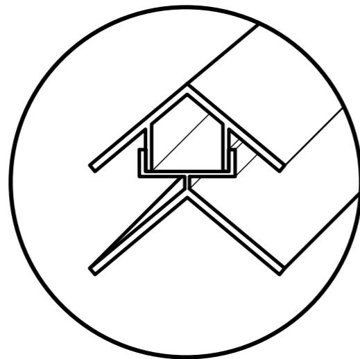
PERFIL INTERIOR SIDING METAL
